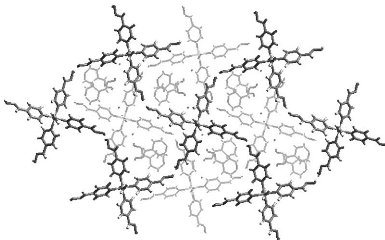
Fig. 14. Part of the 3D structure of 24. Dark gray metal complexes represent one hydrogen-bonded layer. Light gray metal complexes are crystallographically-equivalent layers below. Additional 4-pyridine aldoxime molecules (light gray) reside in channels.
